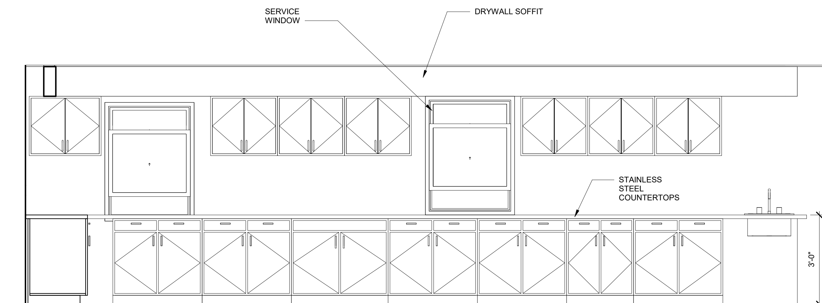
6 ELEVATION-KITCHEN SCALE: 1/2" = 1'-0"
