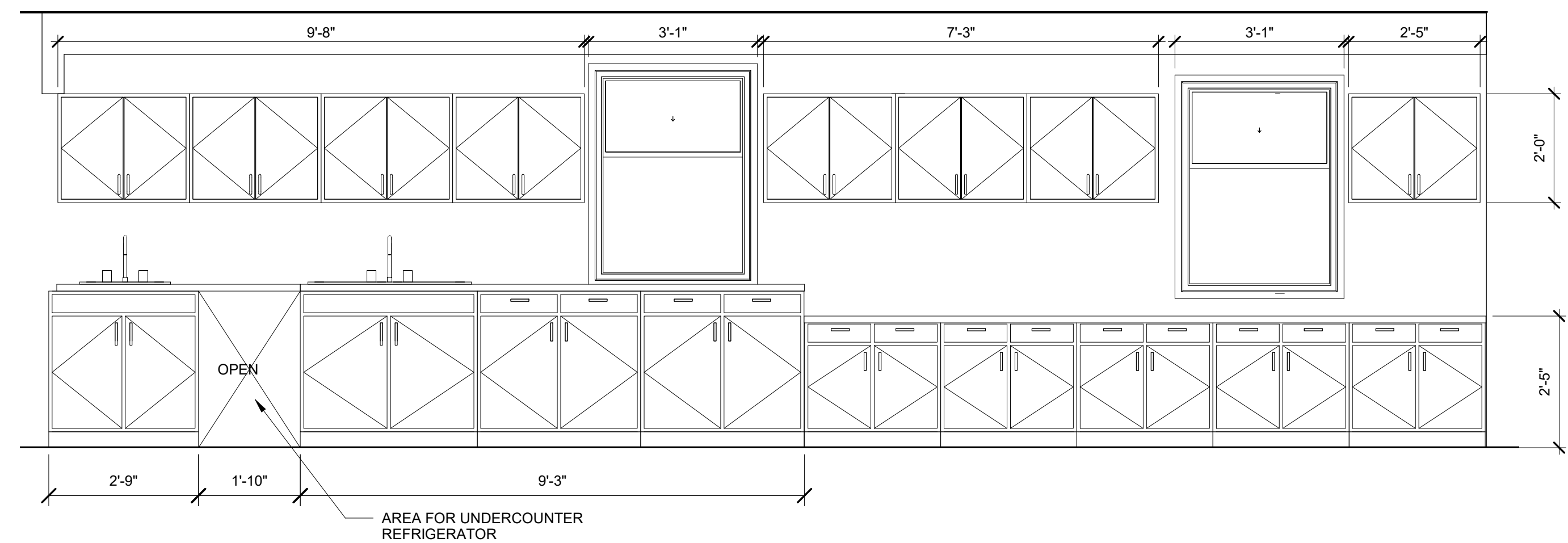
4 ELEVATION- DEMO KITCHEN SCALE: 1/2" = 1'-0"
